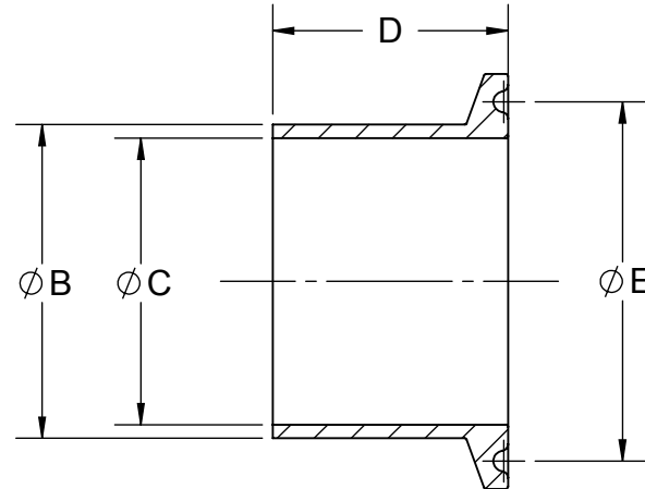
SECTION Y-Y
